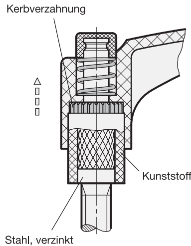
ELESA Original design: ERX.p
